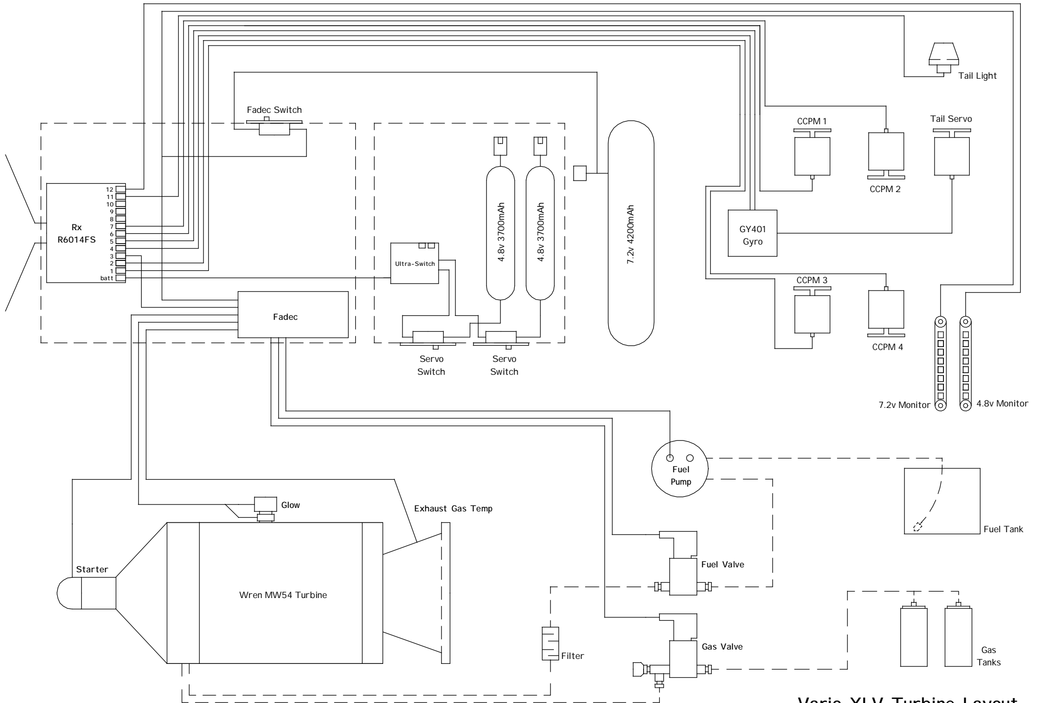
Vario XLV Turbine Layout
